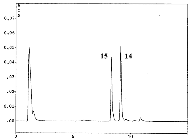
Figure 1. Crude HPLC chromatogram after treatment of 13 with aqu. ammonia at 50 °C for 16 h
