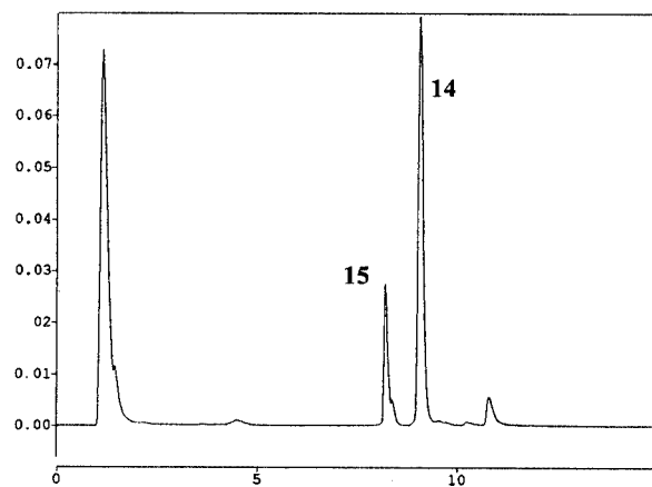
Figure 2. Crude HPLC chromatogram after treatment of 13 with aqu. ammonia at room temperature for 16 h
