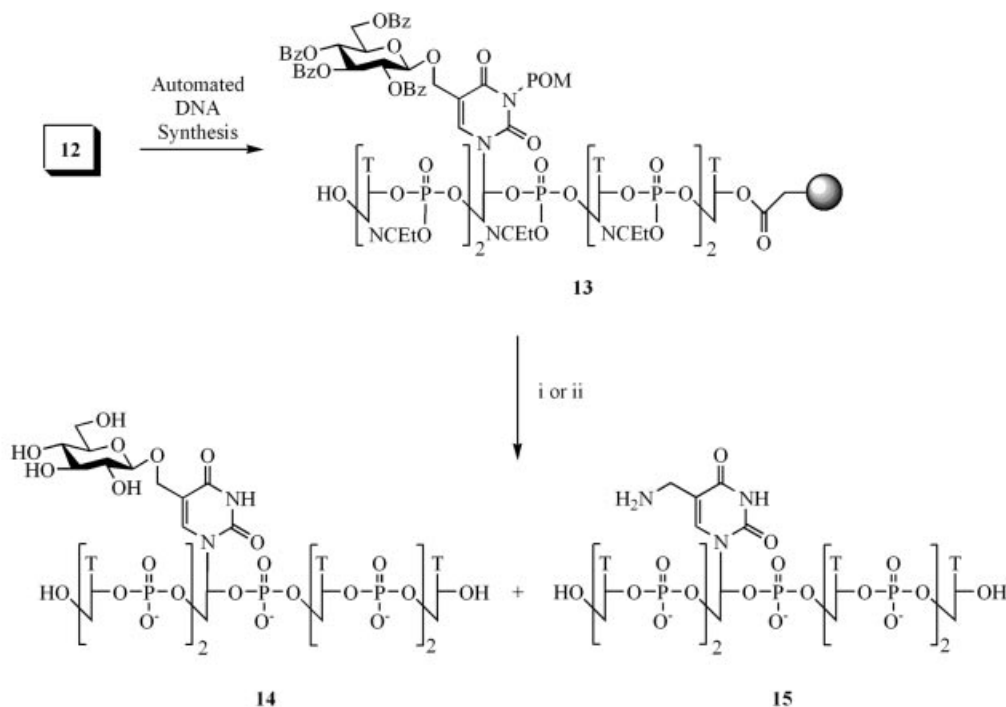
Scheme 2. Reagents and conditions: (i) \text{NH}_3 (aq.), 50 °C, 16 h, 14/15 = 3:2 (see Figure 1); (ii) \text{NH}_3 (aq.), room temp., 16 h, 14/15 = 4:1 (see Figure 2)
