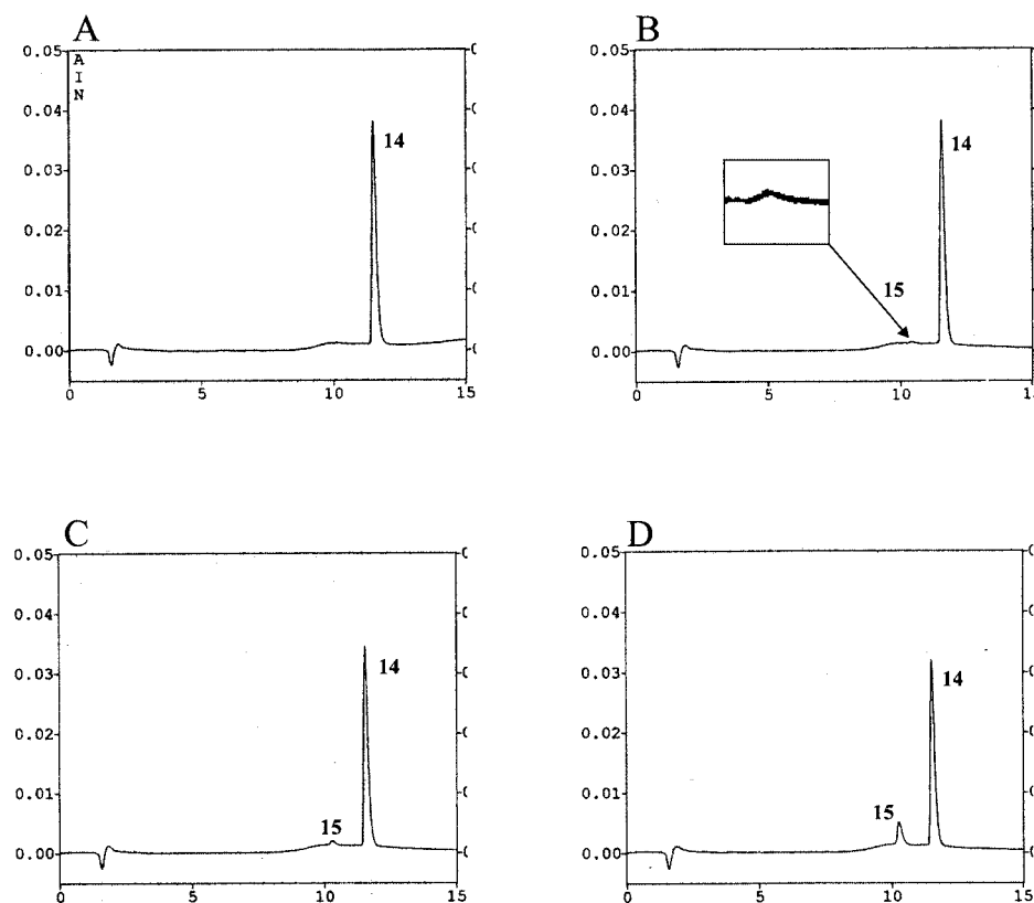
Figure 3. (A) Pure 14 , obtained by preparative RP-HPLC; (B) 14 after \text{NH}_3 (aq.), room temp. 16 h; (C) 14 after \text{NH}_3 (aq.), room temp. 64 h; (D) 14 after \text{NH}_3 (aq.), 50 °C, 16 h
