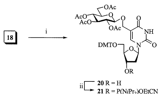
Scheme 4. Reagents and conditions: (i) DMTCl, py, room temp., 16 h, 90%; (ii) CIP( \text{NiPr}_2 )OEtCN, DIPEA, DCM, room temp., 96%
